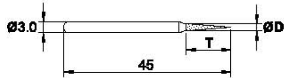
BM Series - \phi 3.0mm shank
