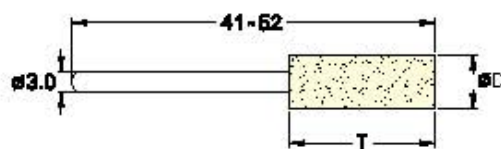
Felt Bobs - \phi 3.0mm Shank
