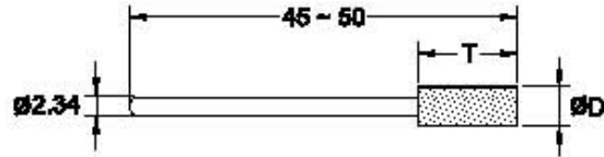
BH Series - \varnothing 2.34 mm shank
